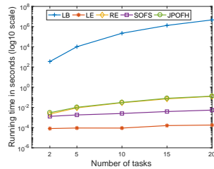
Fig. 3: Effect of number of tasks on running time
