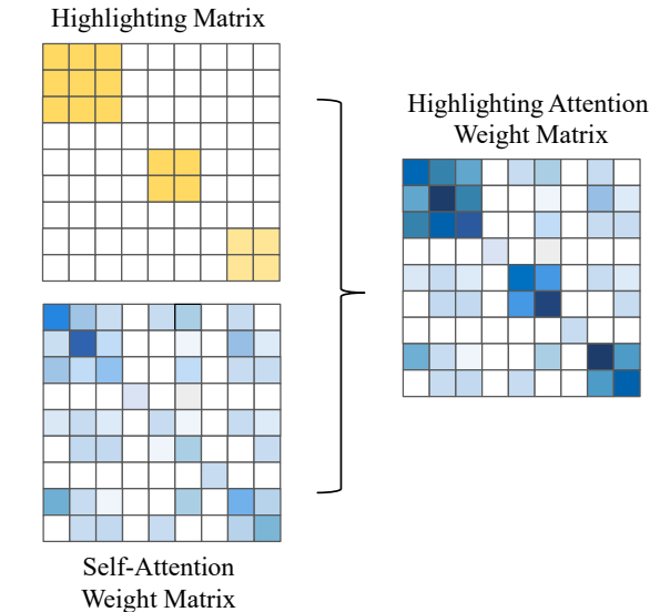
Figure 1: The highlighting mechanism assigns greater attention weights for tokens within key phrases indicated by the highlighting matrix.
