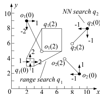
Fig. 1 Examples of spatiotemporal data and queries
