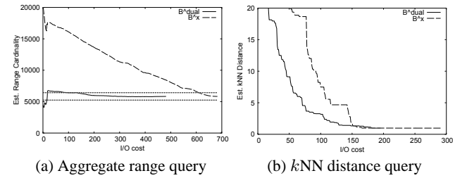
Fig. 22 Progressive query estimates
