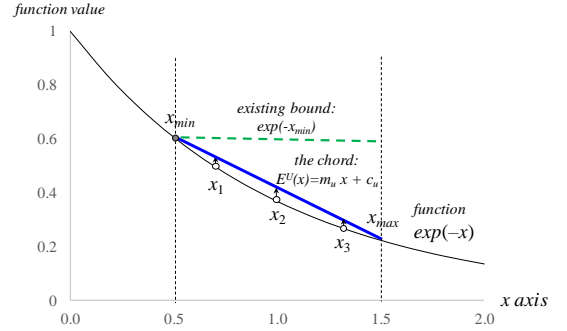
Fig. 4: Chord-based upper bound function
