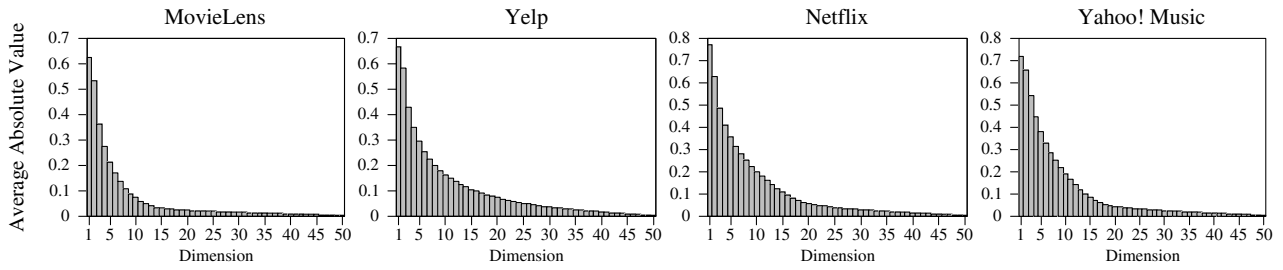
Figure 19: Value Distributions of Reordered p
