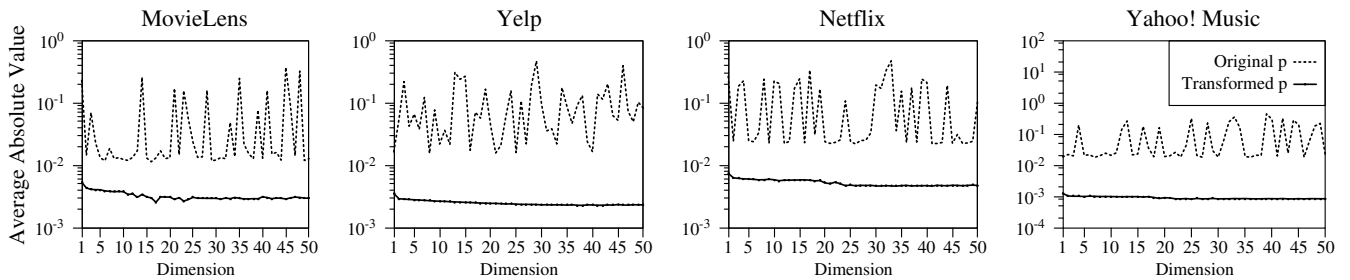
Figure 17: Value Distributions of p Before and After SVD Transformation
