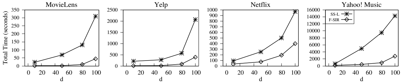
Figure 20: Total Retrieval Times for All Queries (Varying d )
