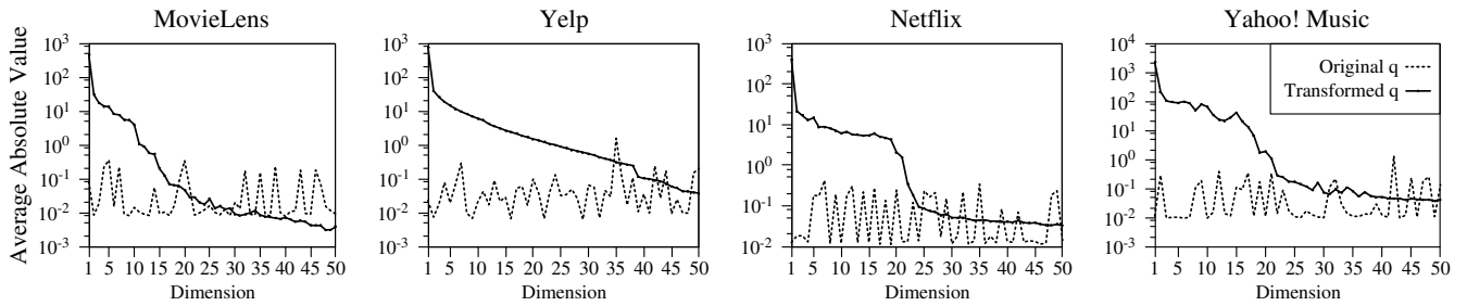
Figure 16: Value Distributions of q Before and After SVD Transformation
