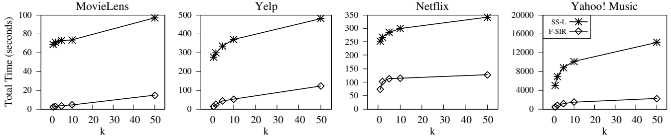
Figure 7: Total Retrieval Times for All Queries (Varying k )
