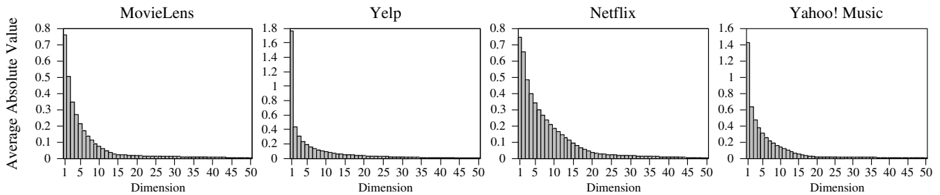
Figure 18: Value Distributions of Reordered q
