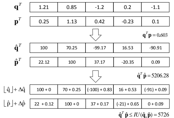
Figure 5: Integer Upper Bound After Scaling
