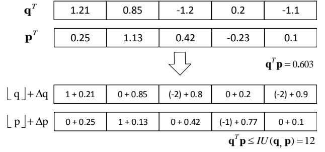
Figure 4: An Example of Integer Upper Bound
