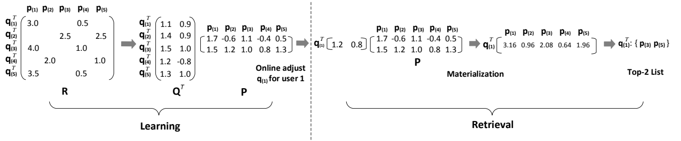
Figure 1: Overview of Top- k IP Retrieval in Recommender Systems Based on Matrix Factorization (MF)
