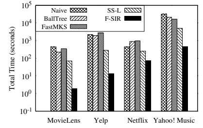
Figure 6: Total Cost ( k=1 )
