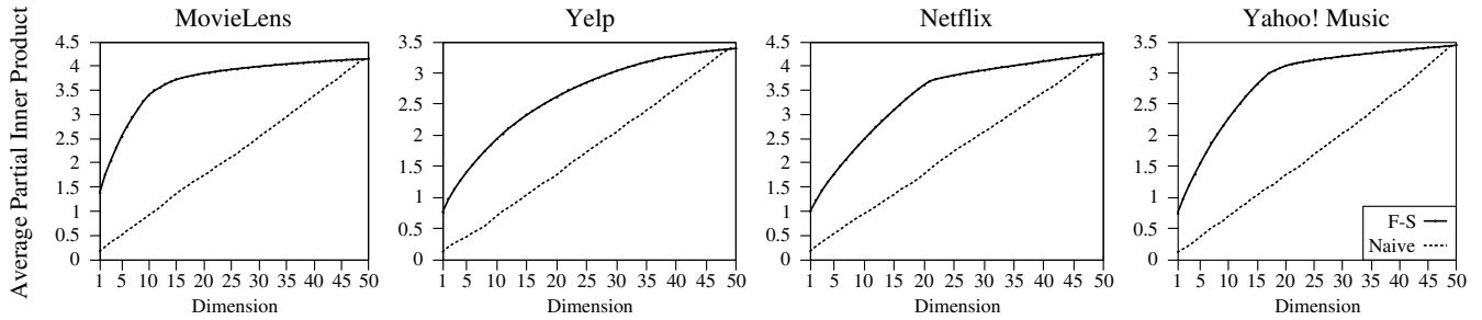
Figure 15: Partial Inner Product Before and After SVD Transformation
