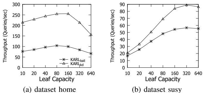
Fig. 7: The throughput of query type I- \tau , varying the leaf node capacity
