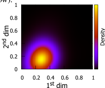
Fig. 1: Kernel density estimation on the miniboone dataset, using 1 st and 2 nd dimensions
